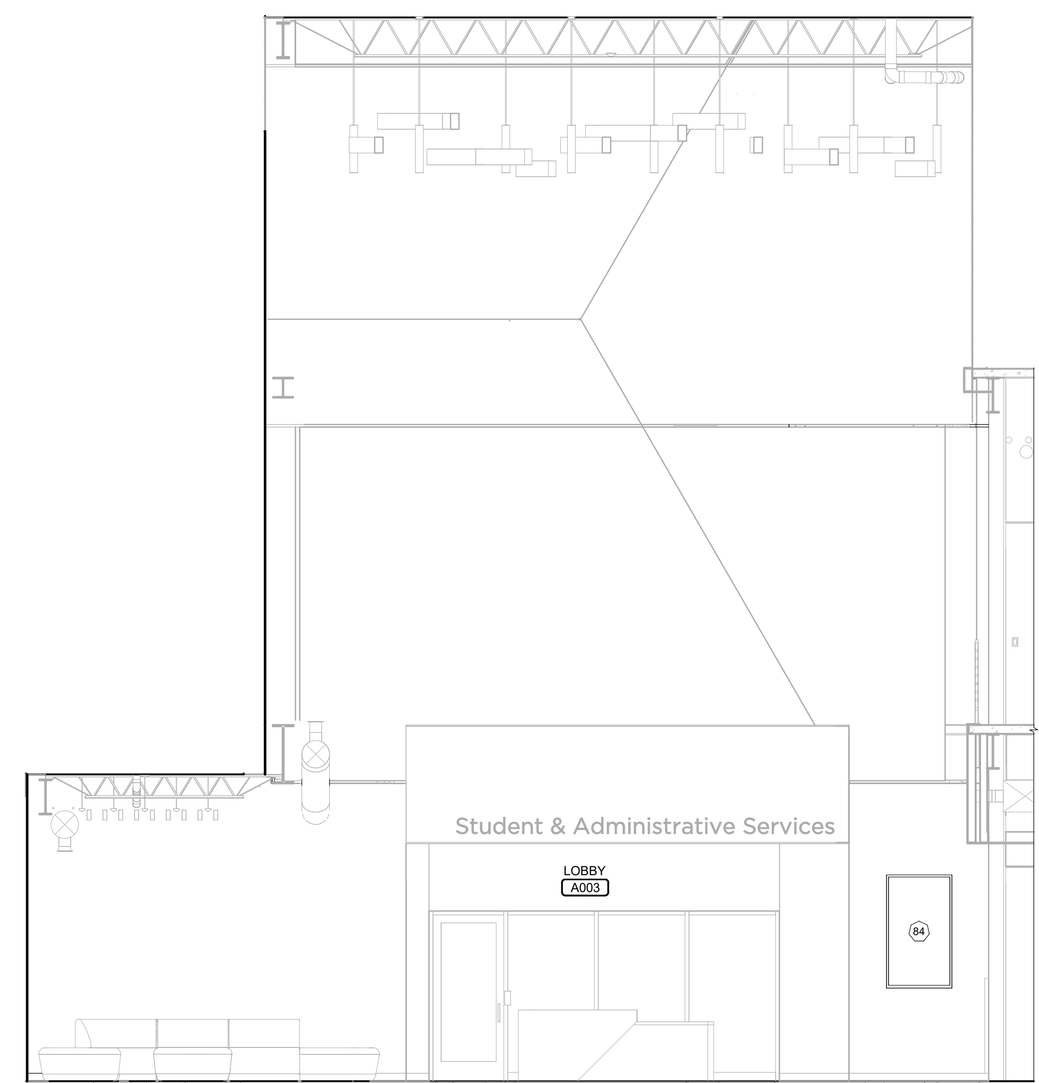
3 LOBBY ELEVATION AT1.3 SCALE: 1/4" = 1'-0"
