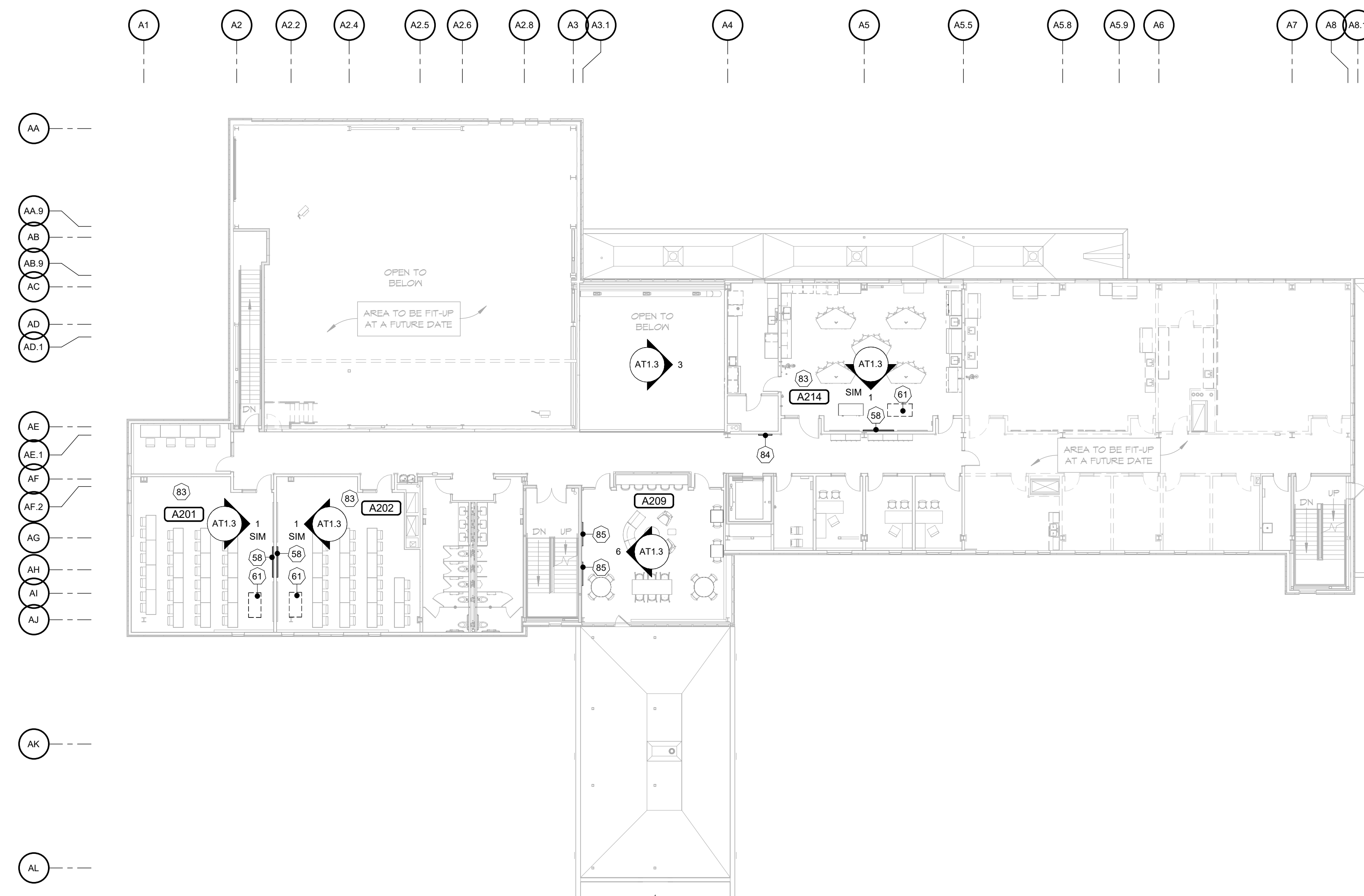
1 SECOND FLOOR TECHNOLOGY PLAN SCALE: 1/16" = 1'-0" 0' 4' 8' 16' 32'
