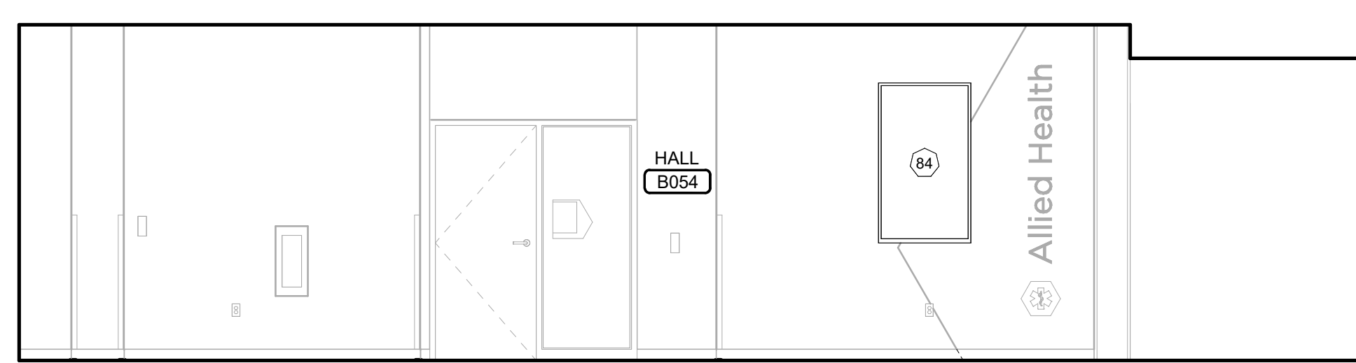
2 HALL ELEVATION AT1.3 SCALE: 1/4" = 1'-0"
