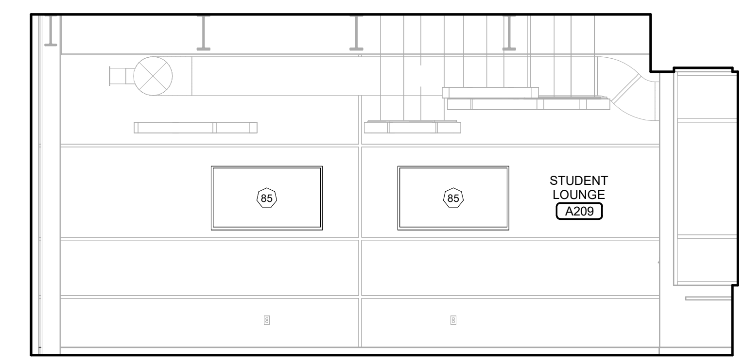
6 STUDENT LOUNGE ELEVATION AT1.3 SCALE: 1/4" = 1'-0"
